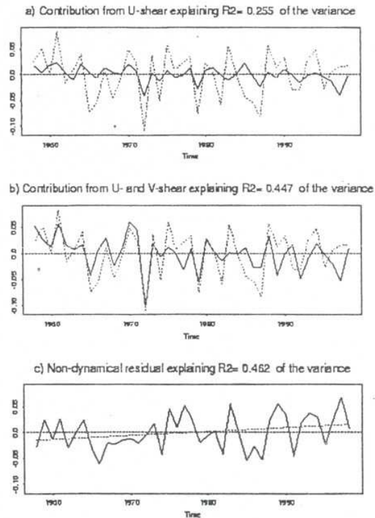
Figs. 2(a-c). Decomposition of the observed P index obtained by performing multiple linear regression : (a) contribution to P from U-shear (solid) with P index (dashed), (b) contribution from both U and V-shears (solid) with P index (dashed), and (c) the residual precipitation not explained by U and V which contains a linear trend (dashed).
