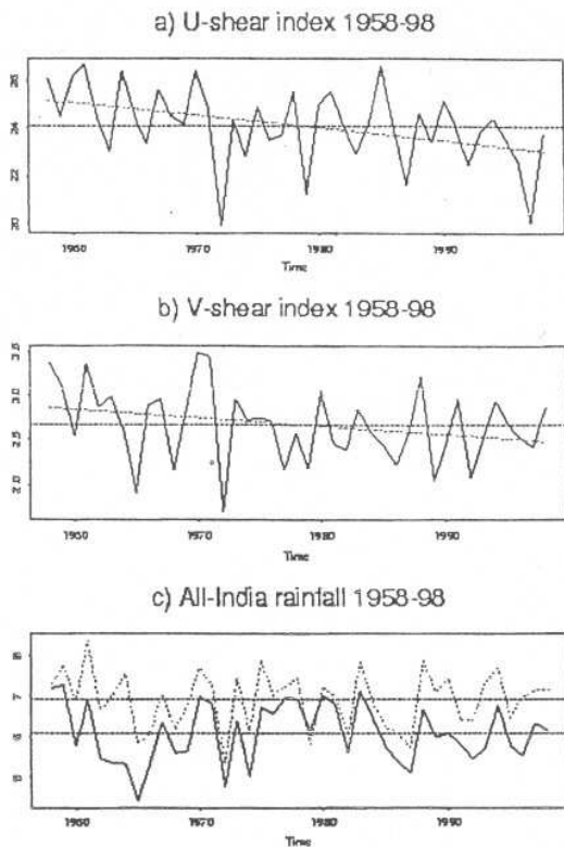
Figs. 1.(a-c). Indices describing the large-scale Asian summer monsoon : (a) mean zonal wind shear index U = u_{200} - u_{850} (m/s) averaged over the domain 40^{\circ} - 110^{\circ} E/EQ- 20^{\circ} N (Webster and Yang 1992), (b) mean meridional wind shear V = v_{200} - v_{850} (m/s) averaged over the domain 70^{\circ} - 110^{\circ} E/10-30 248^{\circ} N (Goswami et al. 1999), (c) summer rainfall averaged over grid points covering India (solid line) and averaged over 306 rain gauges (dashed line). Note the decreasing trends in both U and V but not in P
