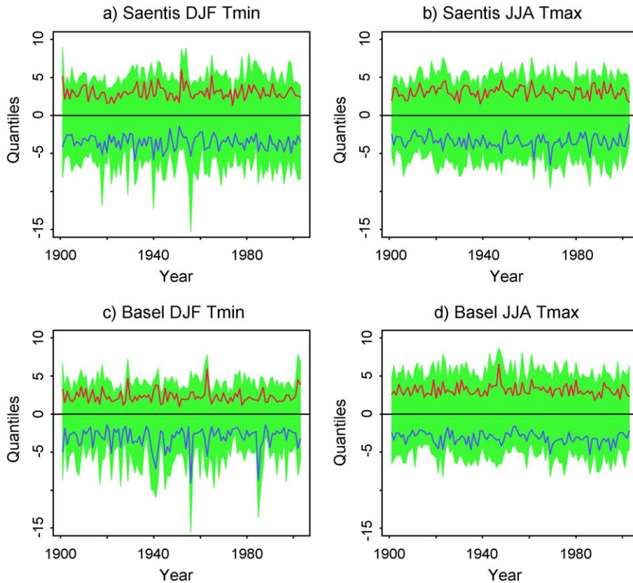
Fig. 3. Time series of the centered 10%, 25%, 50%, 75%, and 90% quantiles for various daily temperature series (in units of ^{\circ}\text{C} ). The quantiles have all been centered by subtracting the 50% quantile (the median) for each season.
