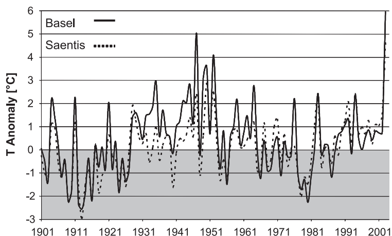
Fig. 5. Anomalies of mean summer maximum temperatures at Basel and Sântis computed as departures from the 1961–1990 mean.
