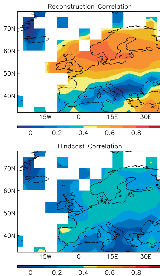
Figure 8. Correlation skill for near-surface temperature reconstructions given perfect predictor data (upper) and hindcasts (lower). Correlations were assessed over 1954–2008. Reconstructed correlation skill uses the observed values of the predictors to assess the maximum amount of variability that can be explained by our predictors. Hindcast skill uses predicted values of the NAO from May SST patterns (RF2002) and other predictors as described in the text.
