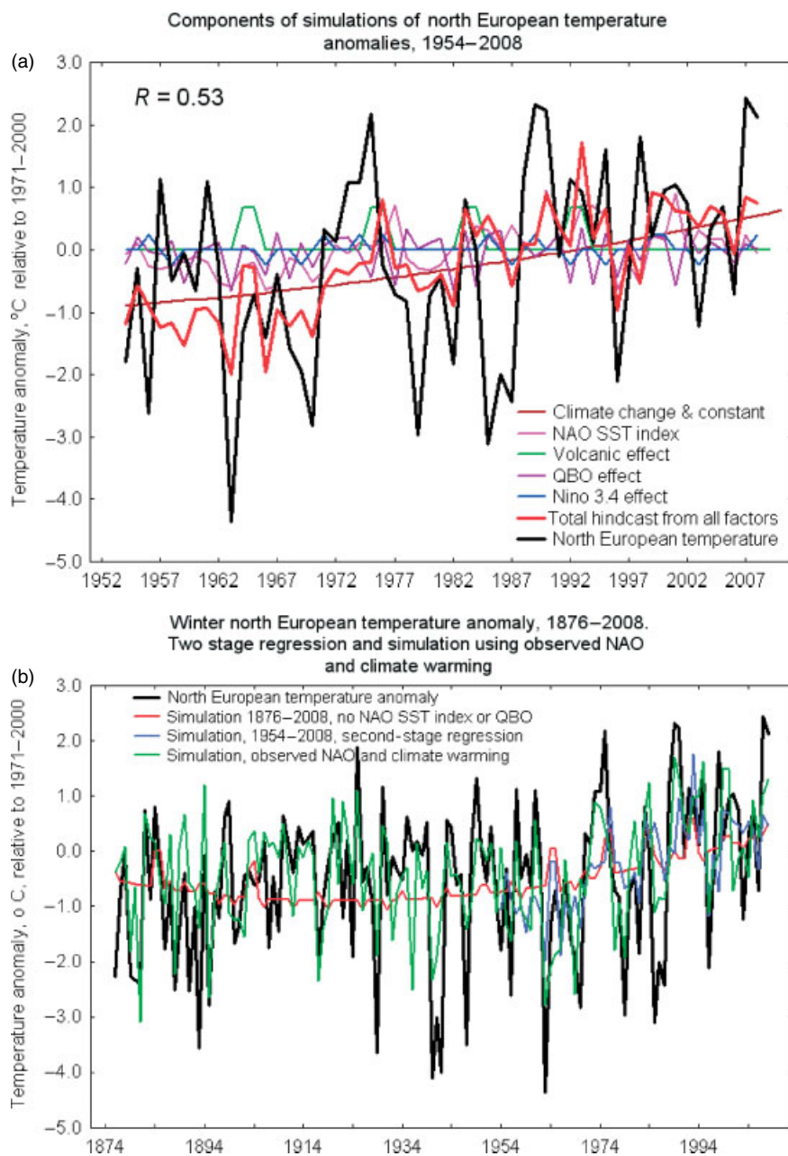
Figure 2. (a) Simulation (no cross-validation) of north European temperature anomalies, 1954–2008, using one-stage regression. The contribution to the simulated temperature of each predictor is shown together with observed north European temperature (black). (b) Two-stage regression simulations of winter mean north European temperature anomalies, 1876–2008. The red line is the simulation using predictors from 1876, the green line using the observed NAO and climate warming and the blue line using predictors available. (c) Cross-validated multiple regression hindcasts, 1954–2008, for north European winter mean temperature anomalies. Each hindcast is based on a set of predictors calculated from all data except the winter being hindcast and the two years before and after. (d) Residual errors (observed north European temperature minus hindcast) from the cross-validated model and the model including the observed NAO, both for 1954–2008. The latter is based on a regression over the whole period 1876–2008. Note large failures such as 1985.
