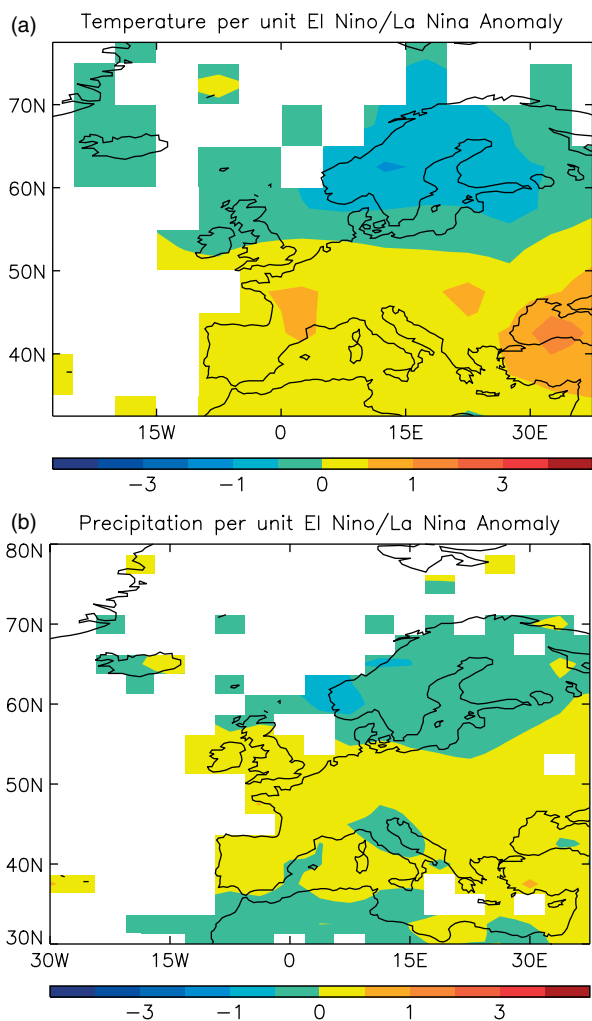
Figure 7. Spatial patterns of predicted (a) temperature, and (b) rainfall over Europe of a positive unit index for an El Nino for temperature and rainfall. This is a fixed anomaly for a (moderate) El Nino with this index value.
