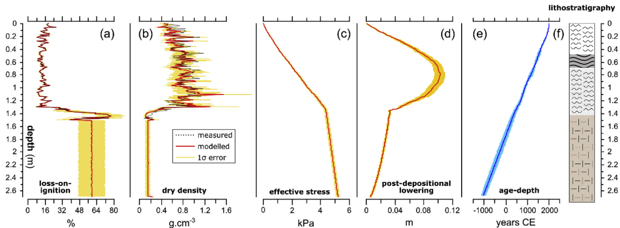
Fig. 9. Physical and geotechnical properties. Measured (black dotted) and modelled (red) \pm 1\sigma (yellow) results of (a) LOI, (b) dry bulk density, (c) effective stress and (d) PDL in monolith SimVII. (e) Age-depth model and (f) lithostratigraphy are also shown. (For interpretation of the references to colour in this figure legend, the reader is referred to the Web version of this article.)
