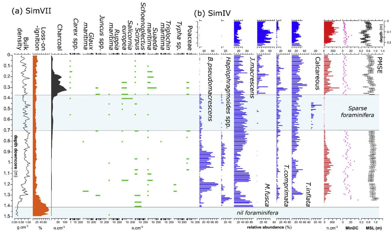
Fig. 6. Palaeoenvironmental analyses. Foraminifera assemblages (blue) are shown as relative abundance for monoliths SimVII (a) and SimIV (b) with corresponding sample test concentrations (red), modern analogue determinations (MinDC) and palaeo-surface elevation predictions (PMSE). Also shown are plant macrofossil concentrations (green), a microcharcoal record (grey) and lithological properties (bulk density and LOI) for monolith SimVII. (For interpretation of the references to colour in this figure legend, the reader is referred to the Web version of this article.)
