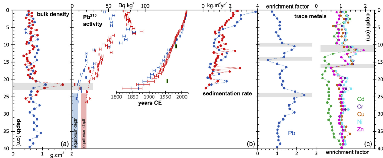
Fig. 7. Geochemical profiles. (a) Dry bulk density measurements of monoliths SimVII (blue) and SimIV (red) with influx of coarse grained sediment highlighted (light grey). (b) Radionuclide ( ^{210}\text{Pb} ) activity and modelled age-depth profiles following Appleby (2001) with calibrated post-bomb radiocarbon ages (black rectangles) and modelled sedimentation rates for monoliths SimVII (blue) and SimIV (red). (c) Trace metal markers for monolith SimVII calculated as enrichment factors (see text for details) with features highlighted as chronohorizons for comparison with the age-depth model for monolith SimVII (light grey). (For interpretation of the references to colour in this figure legend, the reader is referred to the Web version of this article.)
