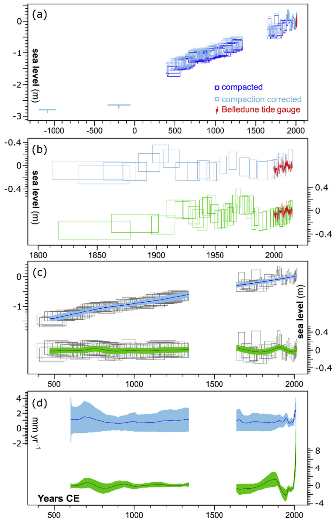
Fig. 10. Reconstructed sea-level data. (a) Late Holocene sea-level reconstruction data from monolith SimVII showing solutions prior to (dark blue) and posterior to (light blue) PDL modelling and compaction correction. Also shown are two basal sea-level index points from Saint-Siméon and the available tide-gauge data from Belledune, New Brunswick (red). (b) Validation reconstruction data from monolith SimIV (green) shown against the equivalent reconstruction data from monolith SimVII (blue) with tide-gauge data for comparison (red). (c) Estimation of the secular sea-level trend from monolith SimVII (blue) ( \pm 2\sigma ) and of the residual 'internal variability' (green) ( \pm 2\sigma ). (d) Calculated rates of change from the relative sea-level trends shown in (c). (For interpretation of the references to colour in this figure legend, the reader is referred to the Web version of this article.)
