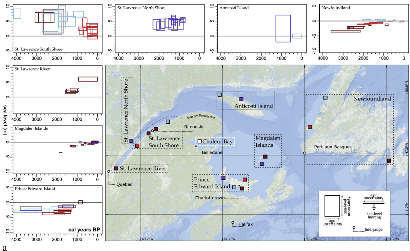
Fig. 1. Location map of eastern Canada and the Gulf of St. Lawrence. The study site in the Baie des Chaleurs (white square) with locations of primary tide-gauge stations (circles) and sources of Late Holocene RSL data (collated by Vacchi et al., 2018) from the St Lawrence Estuary (Dionne, 1990, 1996; 1997, 1999; 2001; Dionne and Coll, 1995; Dyke, 2004), Anticosti Island Dubois et al. (1985), Prince Edward Island (Frankel and Crowl, 1961; Scott et al., 1981), Magdalen Islands (Barnett et al., 2017a) and Newfoundland (Brookes et al., 1985; Wright and van de Plassche, 2001; Daly et al., 2007).
