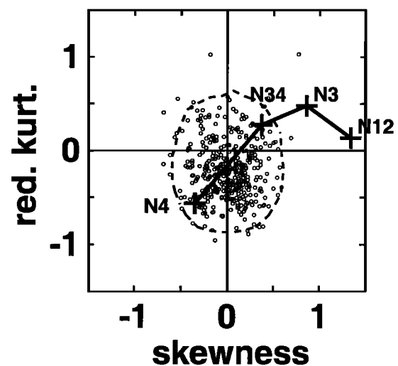
Figure 2. Scatter plot of reduced kurtosis versus skewness estimated for the observed Niño indices over 1950–97 (labeled +). The cloud of points marks values obtained for 400 Monte Carlo realizations of an AR(1) red noise process, with a lag-1 correlation of 0.92. The dashed contour encloses 95% of the Monte Carlo points.
