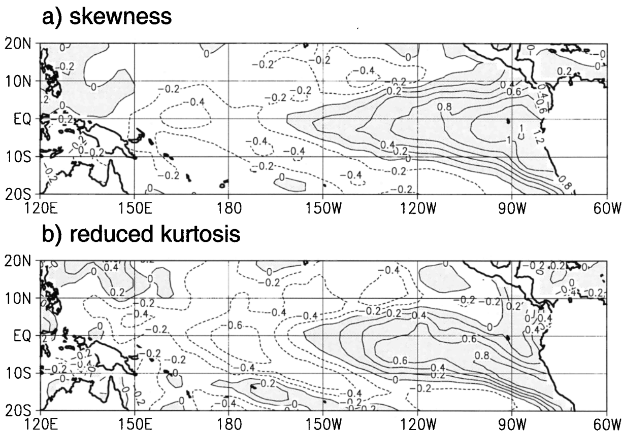
Figure 3. Spatial distribution of a) skewness, and b) reduced kurtosis for the observed monthly mean sea surface temperature anomalies in the Pacific ocean from 1950-97. Note the marked difference between the eastern and western Pacific.
