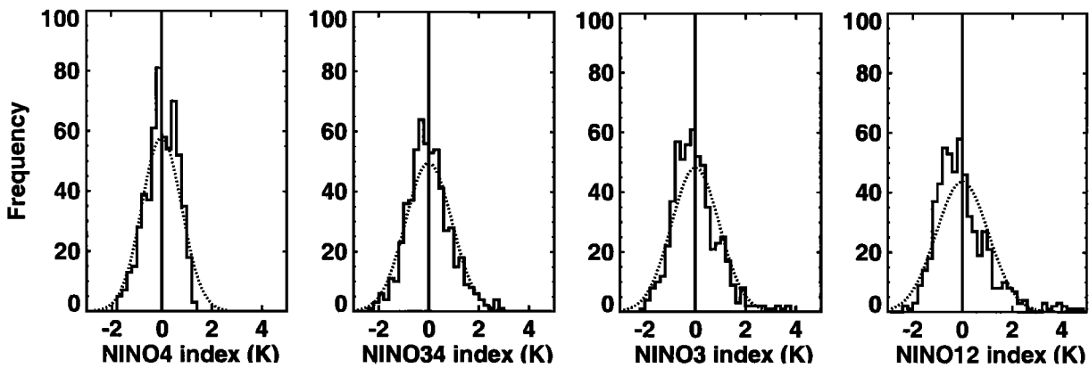
Figure 1. Histograms of the monthly mean Niño index anomalies from 1950–97. For comparison, normal distributions with the observed standard deviation are drawn (dashed line). The mean anomalies are zero by definition. A bin width of 0.2^{\circ}\text{C} was used.
