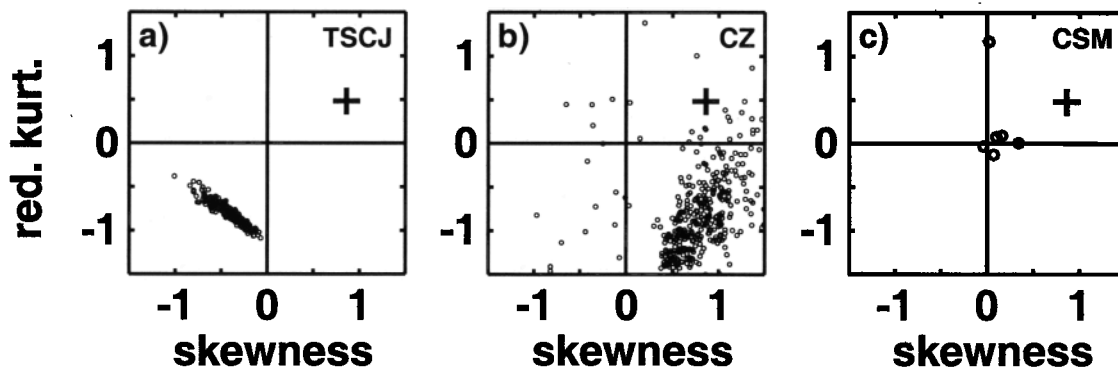
Figure 4. Scatter plot of reduced kurtosis versus skewness of the Niño-3 index in sections of 576 months generated by (a) TSCJ conceptual model, (b) CZ intermediate model, and (c) NCAR CSM global coupled climate model. The value for the observed Niño-3 index over the period 1950-1997 is also shown (labeled +).
